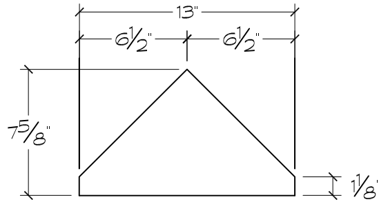
CROSS SECTION
